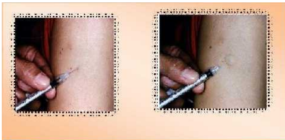
Fig 3.1. ID inoculation
