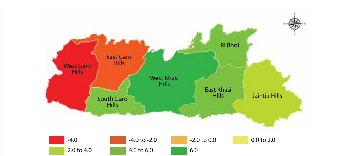
District-wise precipitation trend (mm/day per 100 yr) of southwest monsoon season (June-September) for the period 1971-2005.
