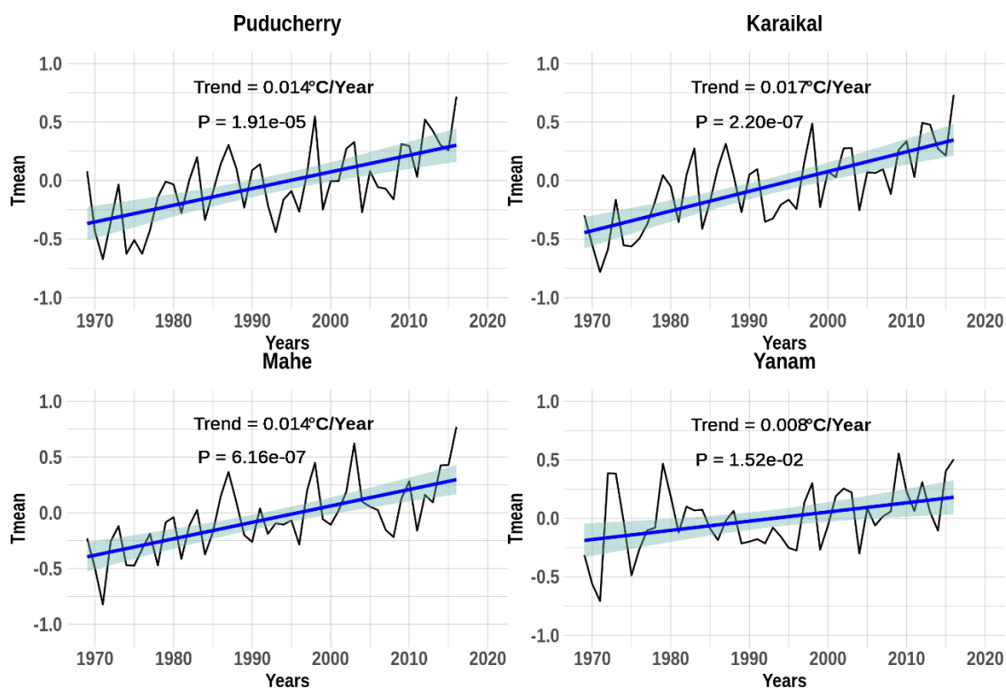
Figure 2: Annual mean temperature anomalies from 1969-2016
