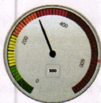
Air Quality Index at Delhi
